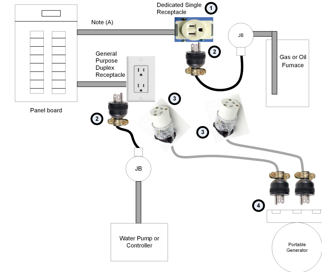
Diagram F1 – Temporary setup for portable generator
