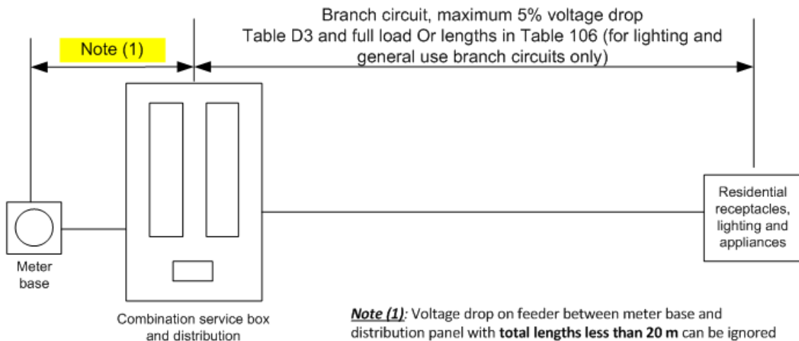
Diagram B2 – Combination service panel
