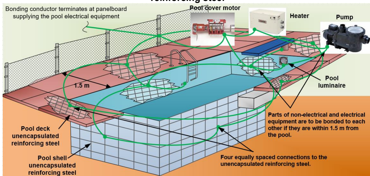
Diagram B1 – Bonding a pool and pool deck with unencapsulated structural reinforcing steel
