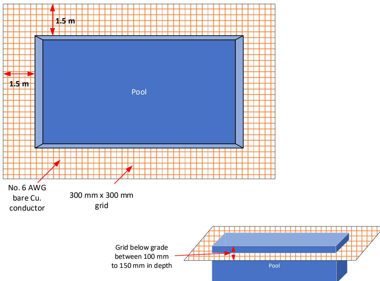
Diagram B3 – Bonding a pool deck with encapsulated structural reinforcing steel
