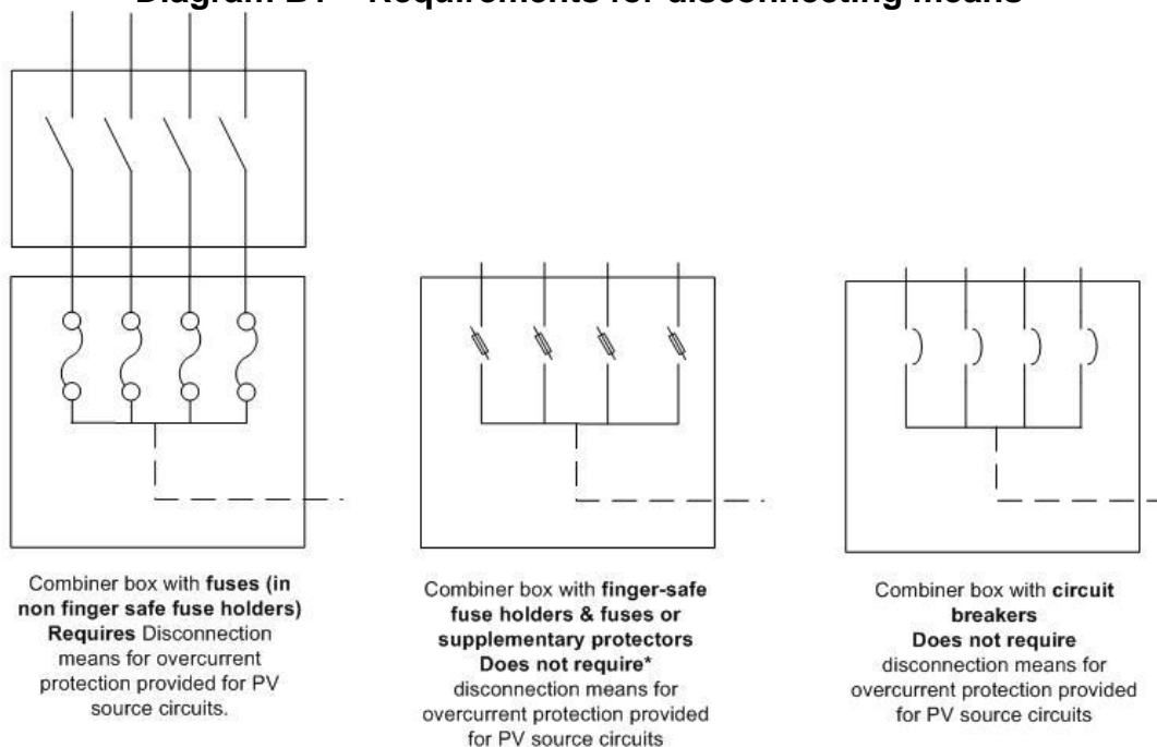
Diagram B1 – Requirements for disconnecting means
