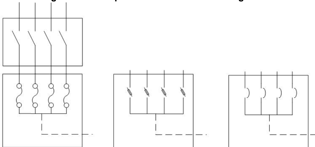
Diagram B1 – Requirements for disconnecting means
