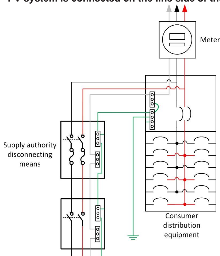
Diagram B1 – PV system is connected on the line side of the service box
