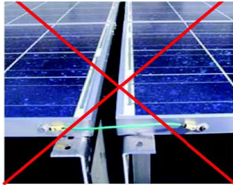
Photo B1 – Unacceptable bonding conductor connection
