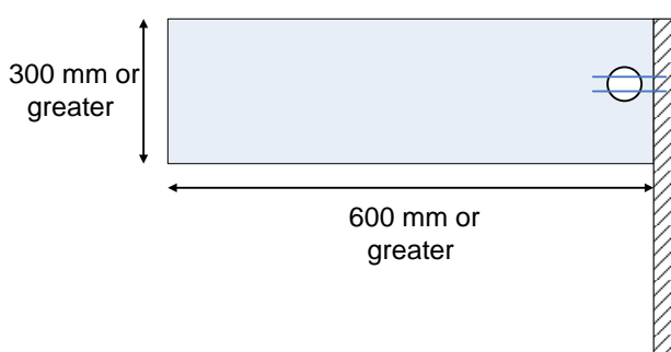
Diagram B5 – Receptacle requirements for a standalone peninsula
