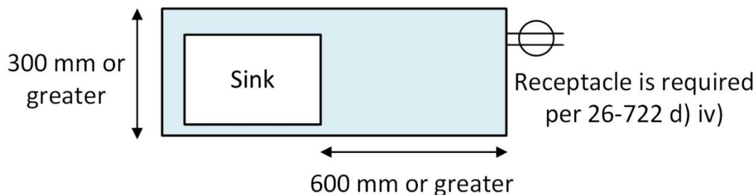
Diagram B1 – Continuous island counter space
