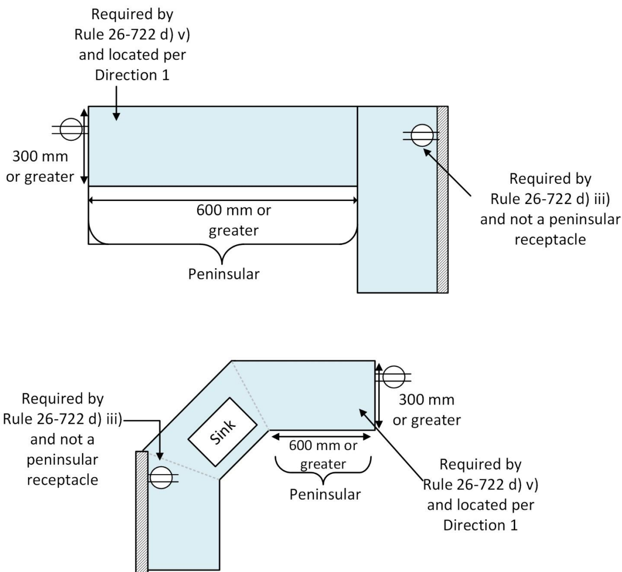
Diagram B4 – Receptacle requirements for a peninsula attached to a kitchen counter
