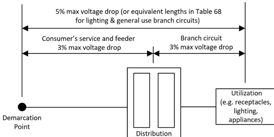
Diagram B2 – Combination service panel located <20m from demarcation point
