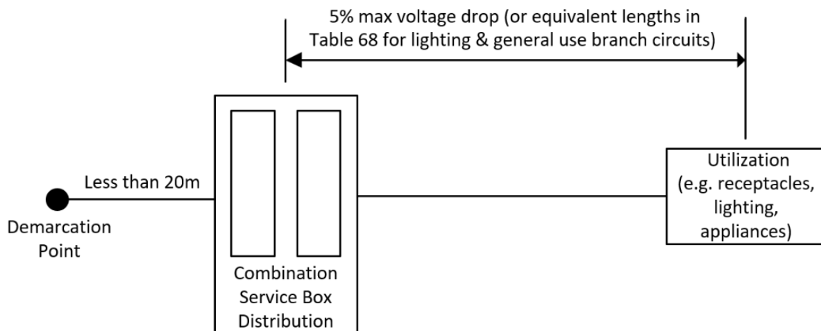
Diagram B2 – Combination service panel located <20m from demarcation point
